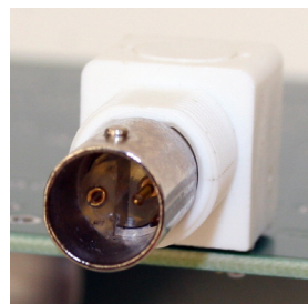
Twin BNC w/ Isolated outer conductor
