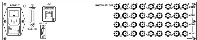
CXAR/32 Rear Panel with IEEE488, RS232 and LAN Control
