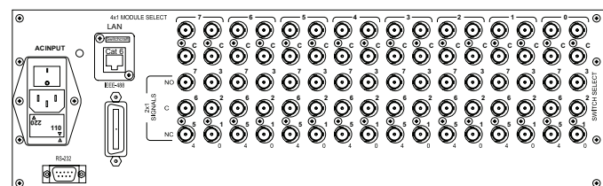
CXAR/64 Rear Panel with IEEE488, RS232 and LAN Control
