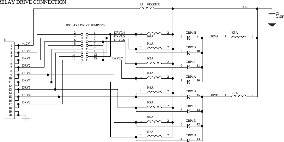
J1 - RELAY DRIVE CONNECTION
