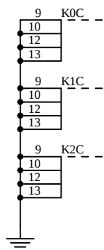
RELAY GROUNDS
