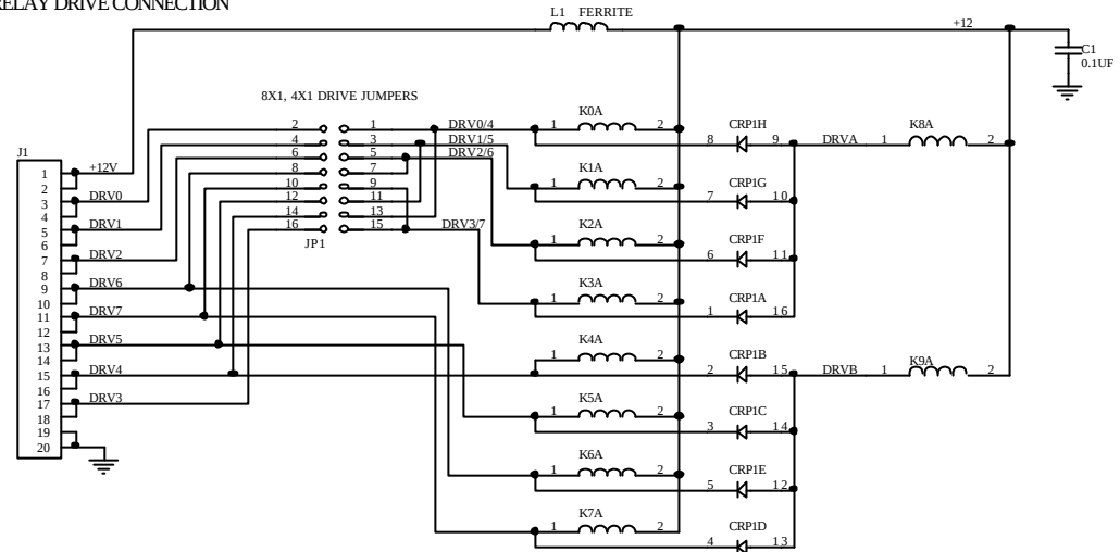
J1 - RELAY DRIVE CONNECTION
