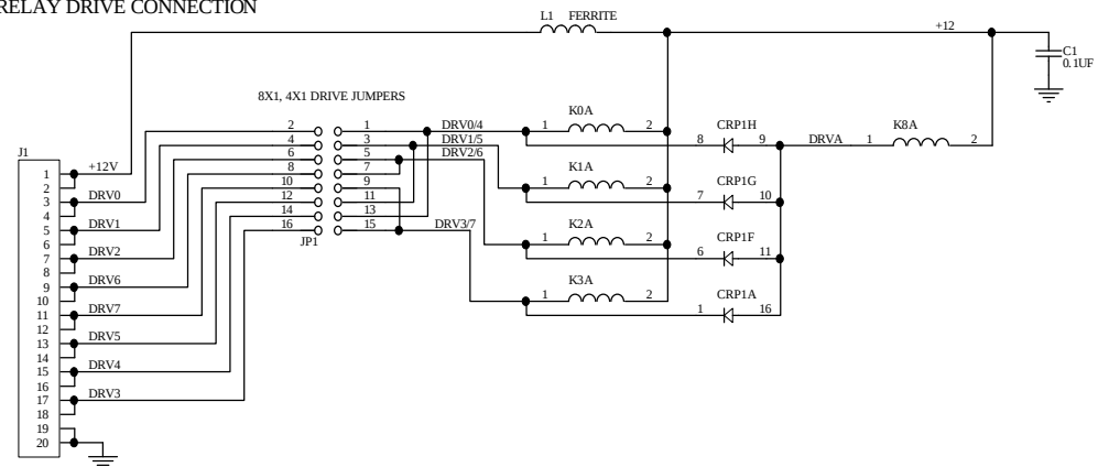
J1 - RELAY DRIVE CONNECTION
