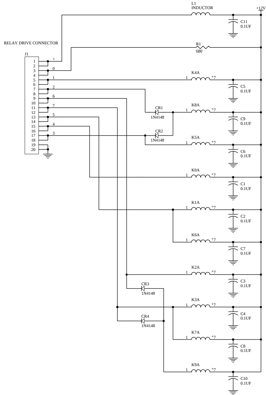
RELAY GROUNDS
