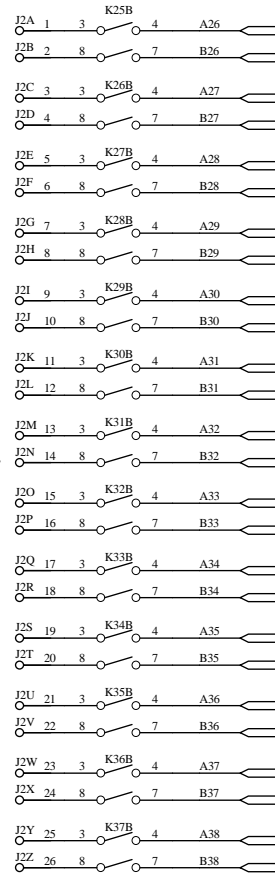
J2 50 Pin Header
