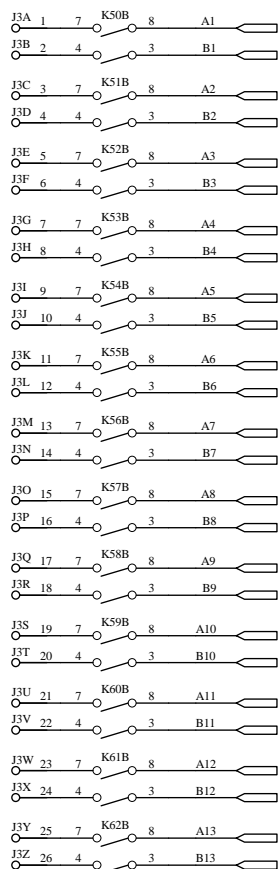
J3 50 Pin Header
