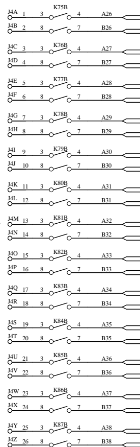
J4 50 Pin Header
