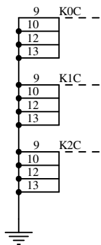
RELAY GROUNDS
