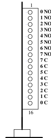
16 PIN SCREW TERMINAL REAR VIEW
