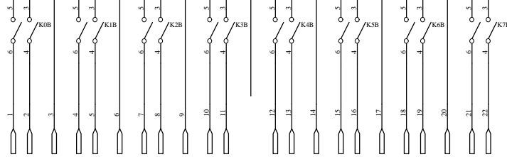
SIGNAL MOTHERBOARD
